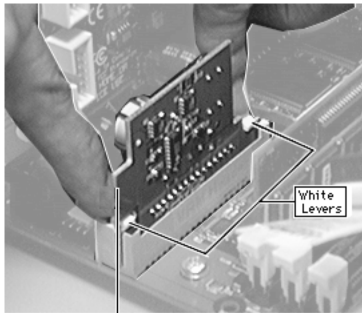
Voltage Regulator
